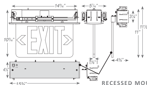
RECESSED MOUNT
