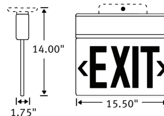
BACK MOUNT
